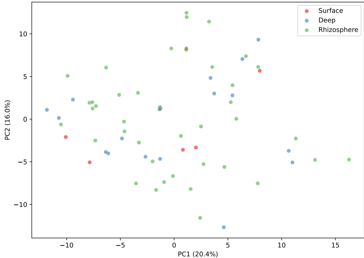
RQ10: PCA of XRF Geochemical Profiles by Compartment
