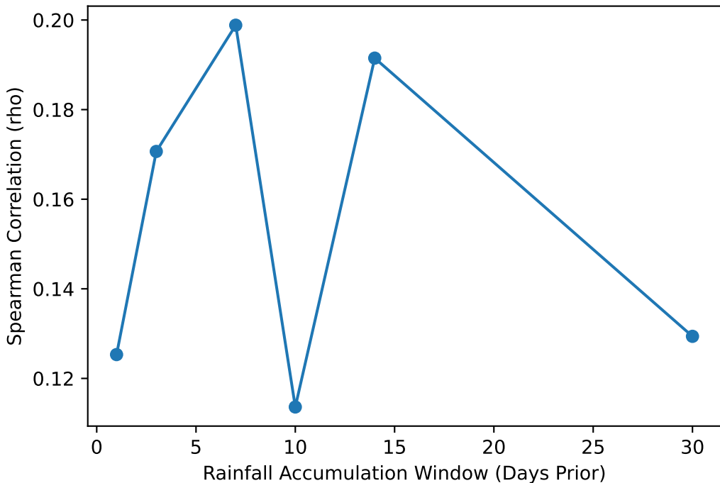
Responder Abundance vs Rainfall Window (Surface)
