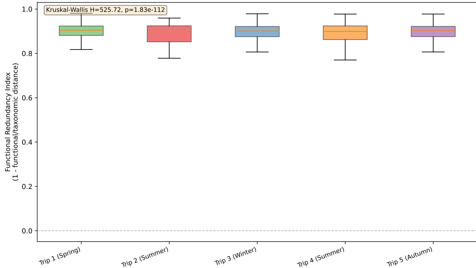
RQ20: Functional Redundancy Index Across Trips
