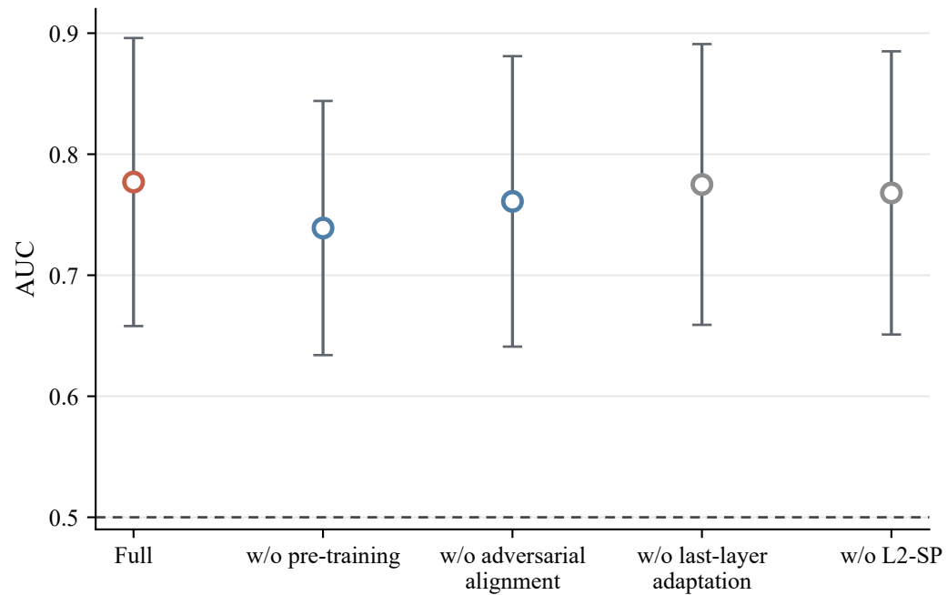
Outer-test AUC across ablation settings
