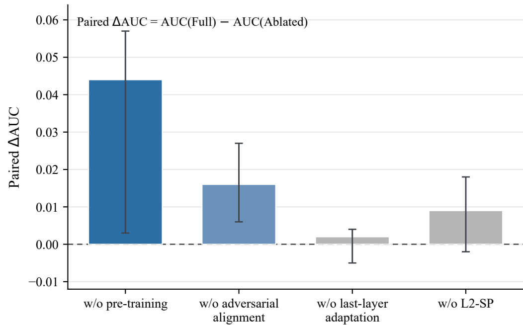
Contribution estimated by paired \Delta AUC
