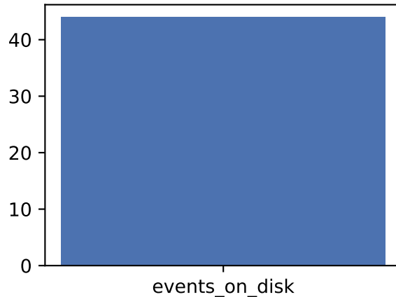
Replay/restart: PASS
