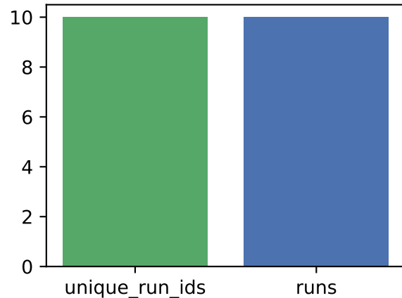
Concurrency: PASS
