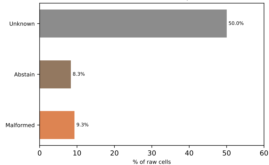
EXP-008: terminal failure mix (valid parse=0.907)
