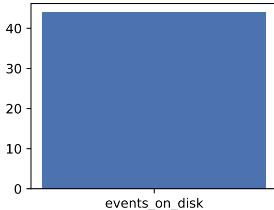
Replay/restart: PASS
