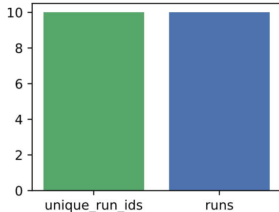
Concurrency: PASS
