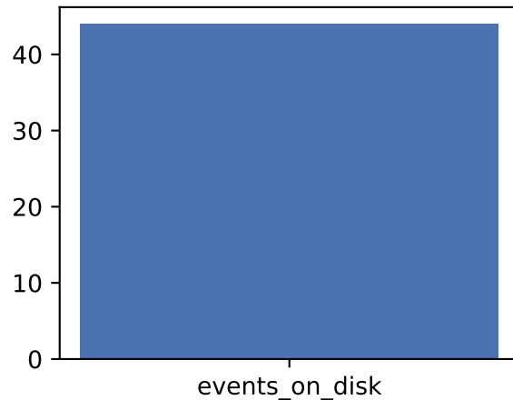
Replay/restart: PASS
