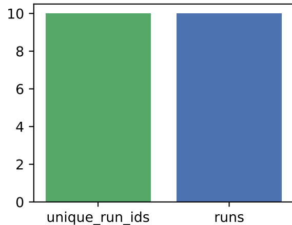
Concurrency: PASS
