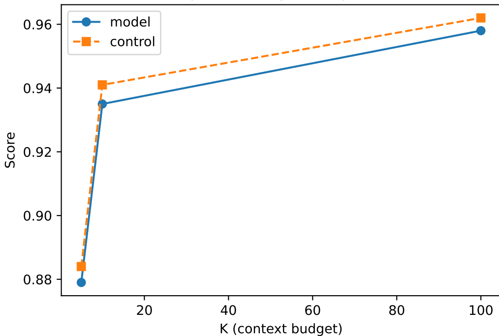
F5: K dose-response (LongMem, qwen2.5-coder-7b)
