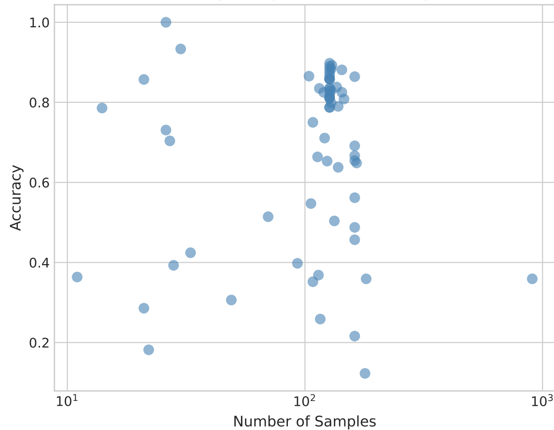
Binary: Sample Size vs Accuracy
