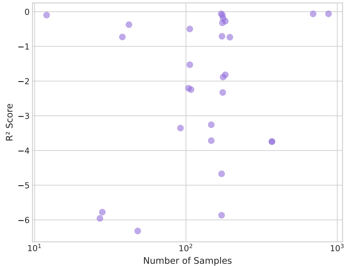
Continuous: Sample Size vs R^2
