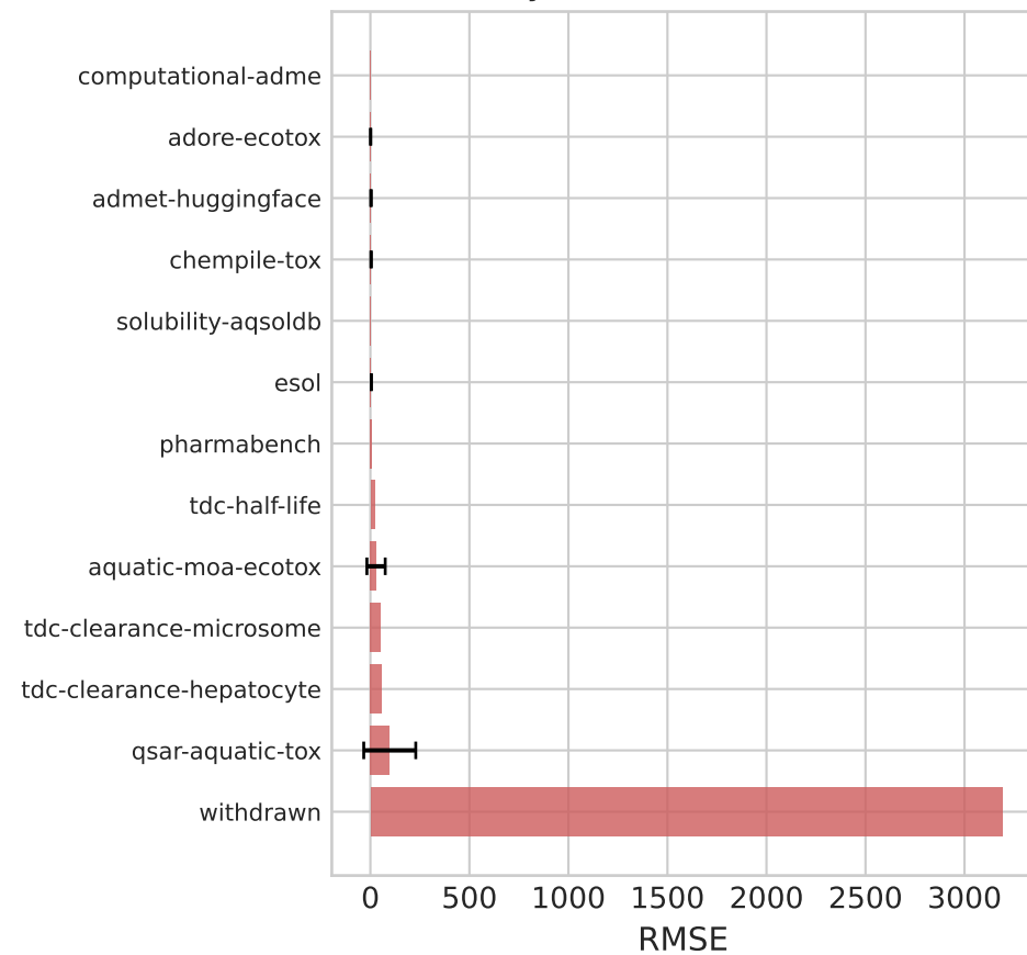
RMSE by Source (lower is better)
