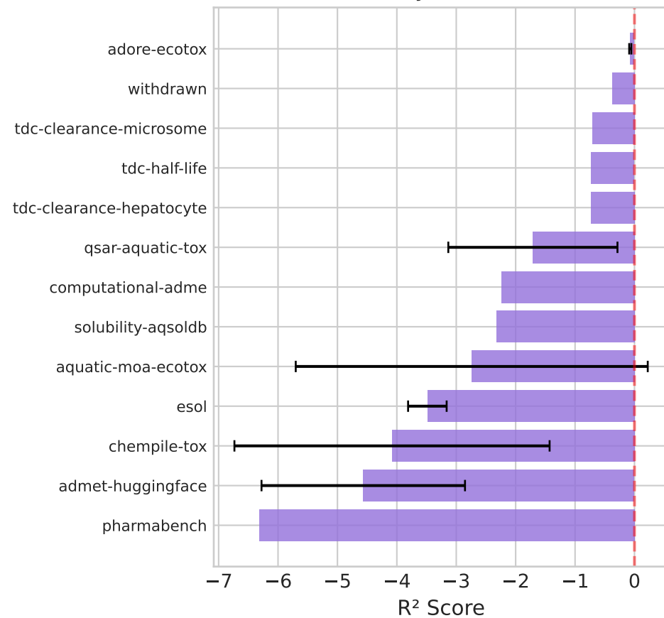
R 2 by Source
