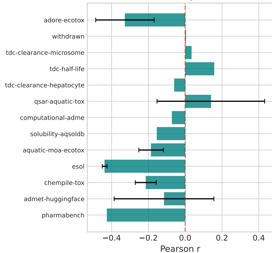
Correlation by Source
