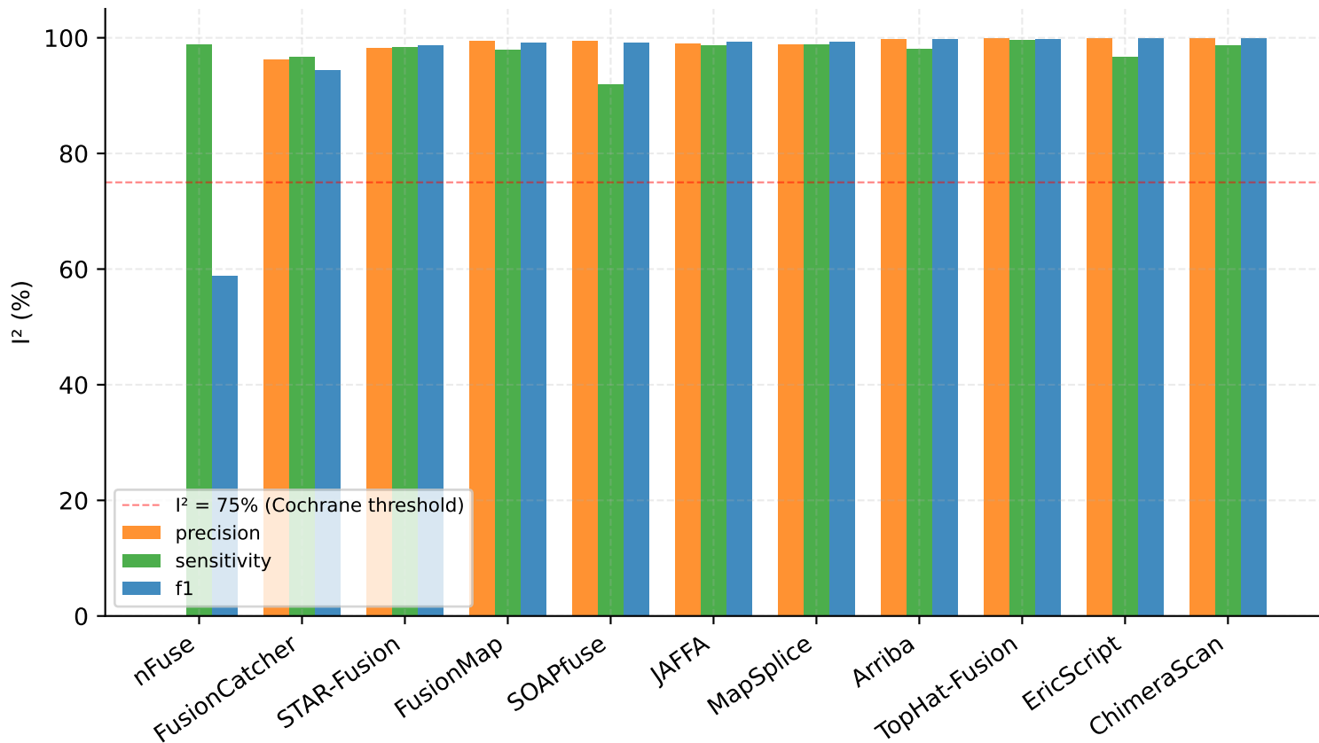
Between-benchmark heterogeneity per tool ( I^2 > 75\% \approx very high; nearly all metrics exceed this)
