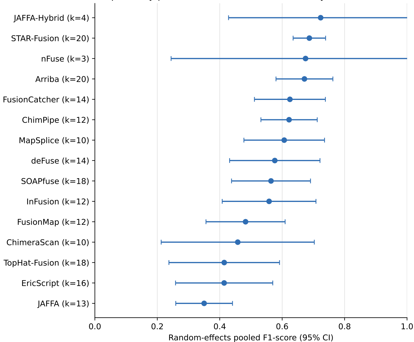
Exploratory pooled F1 estimates for recurrently evaluated tools
