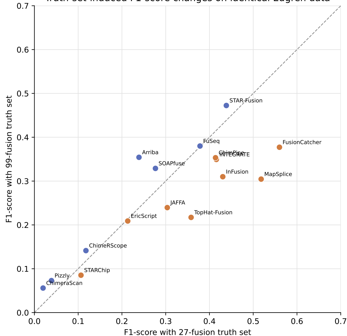
Truth-set-induced F1-score changes on identical Edgren data
