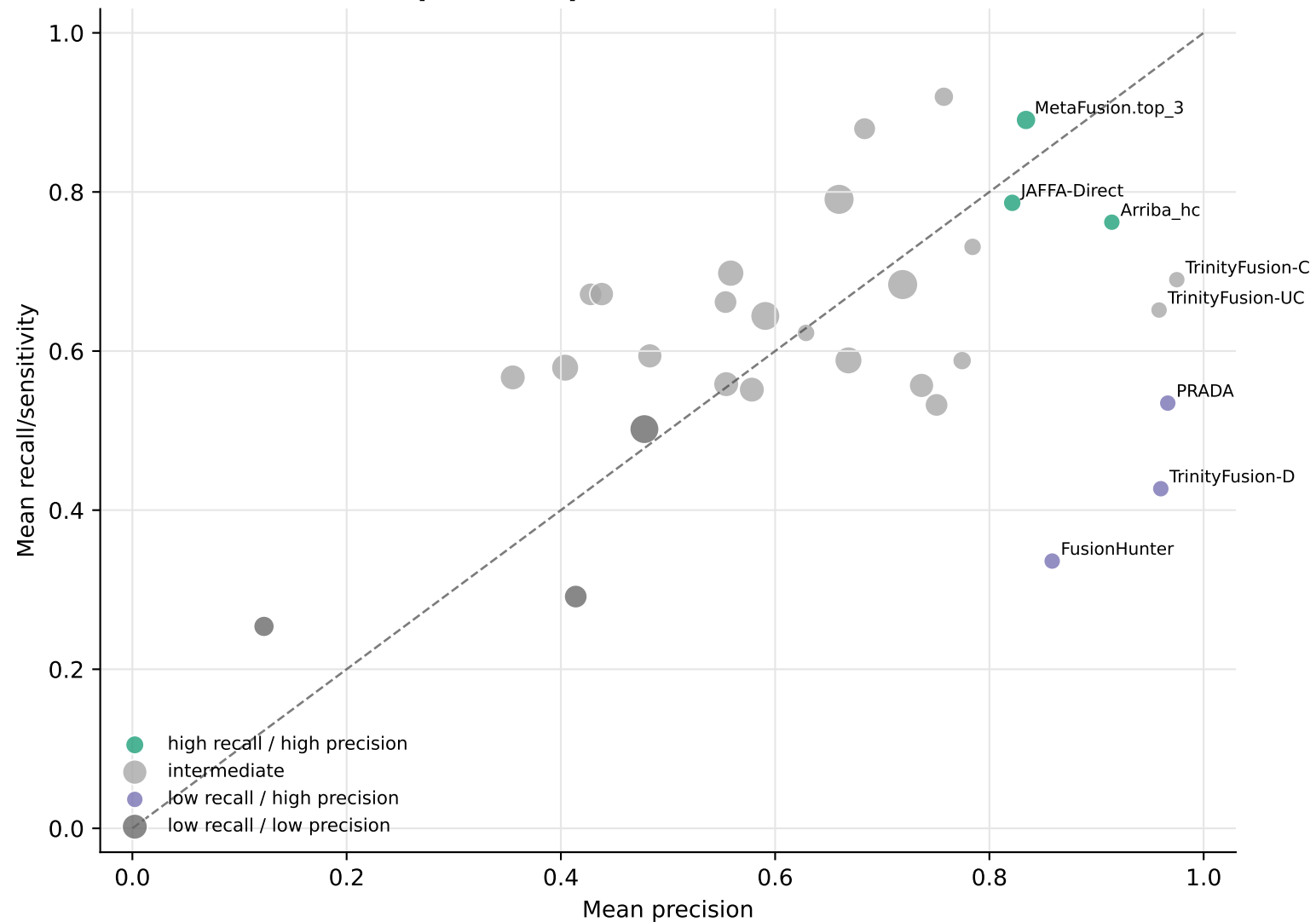
Tool-level recall--precision profiles across benchmark observations
