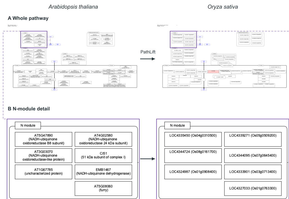
Figure 1: Arabidopsis-to-rice pathway liftover: whole pathway and N-module detail
