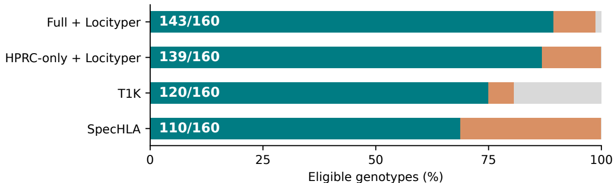
C Assembly SAS: 20 donors, 8 loci
