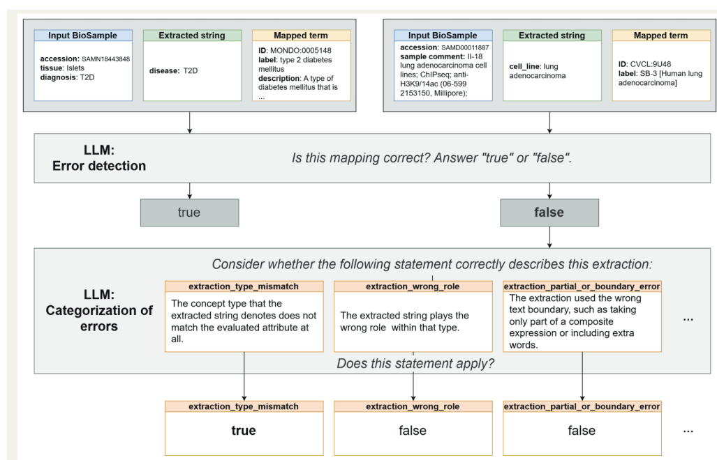
Figure 1: The flowchart of the error detection and categorization process. Error categories are defined in Table 2.
