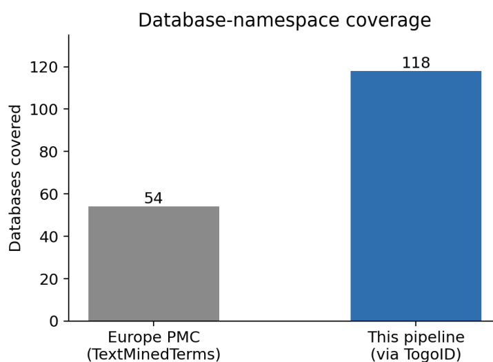
Figure 2: Database-namespaces coverage: Europe PMC's TextMinedTerms vs. this pipeline's TogoID-derived pattern set.
