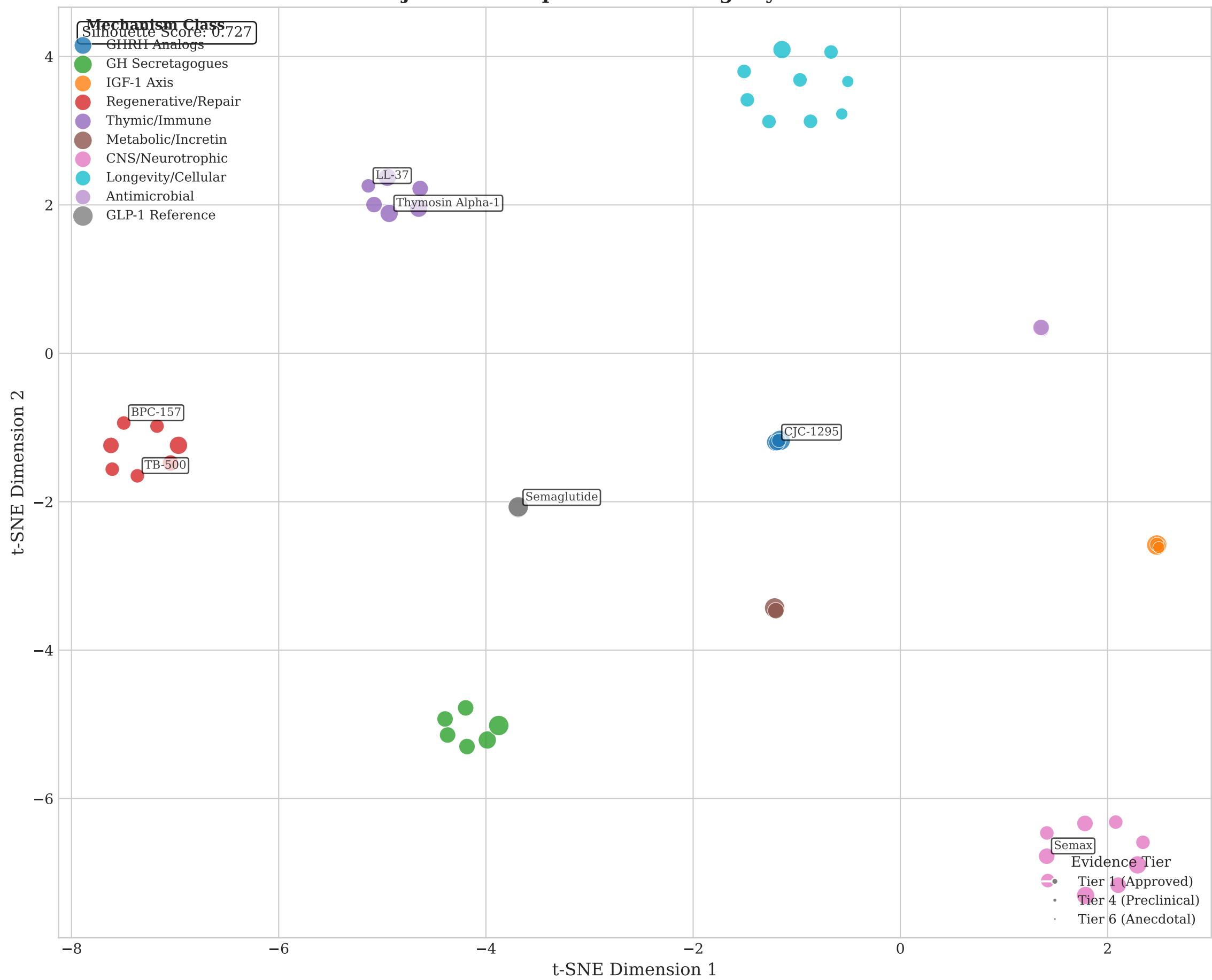
t-SNE Projection of Peptide Embeddings by Mechanism Class
