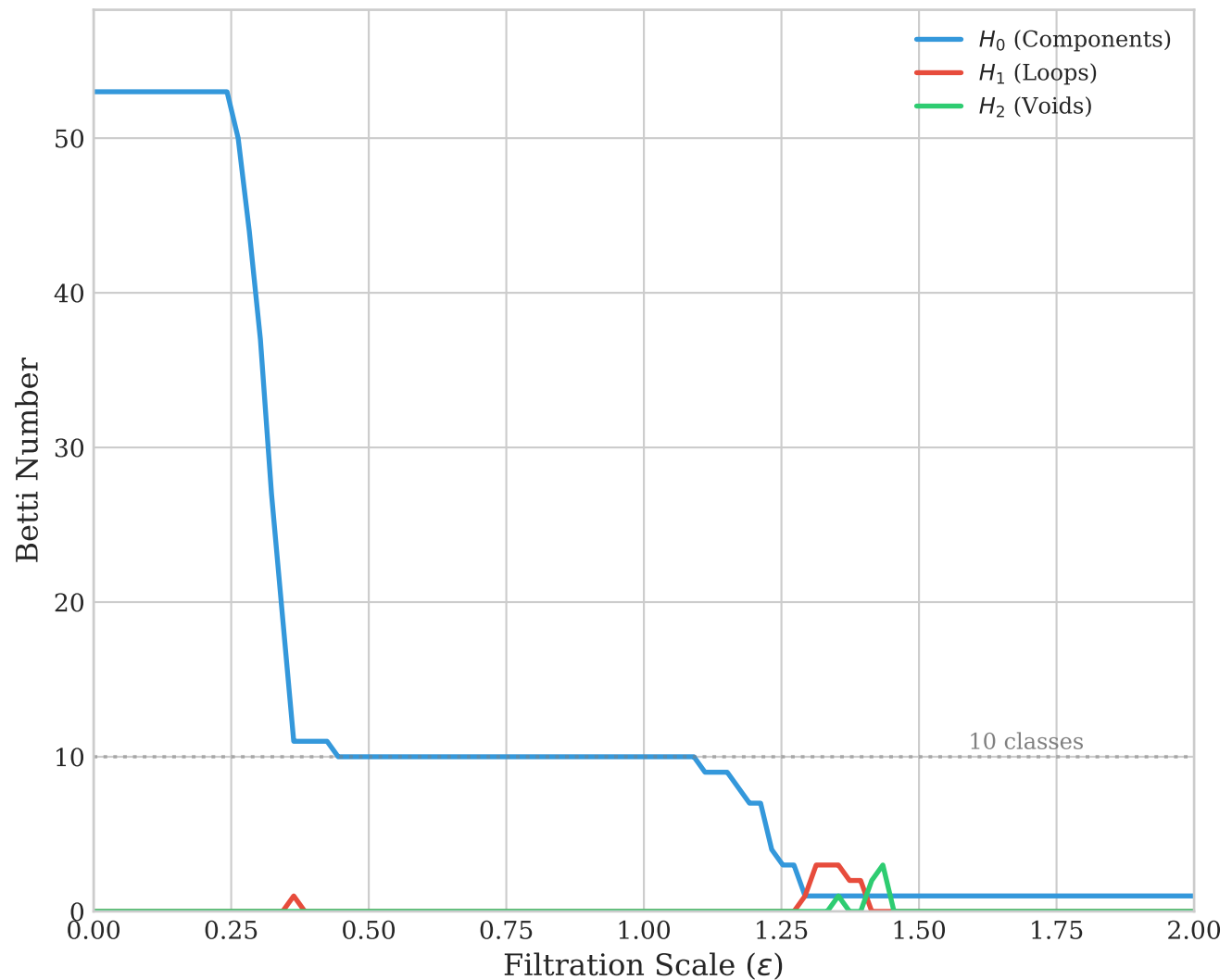
Betti Number Curves
