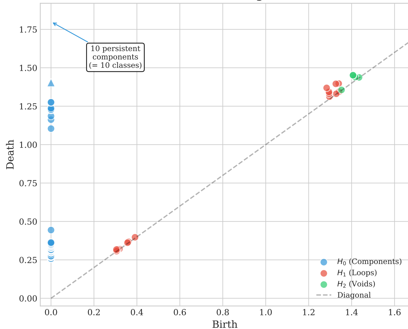
Persistence Diagram
