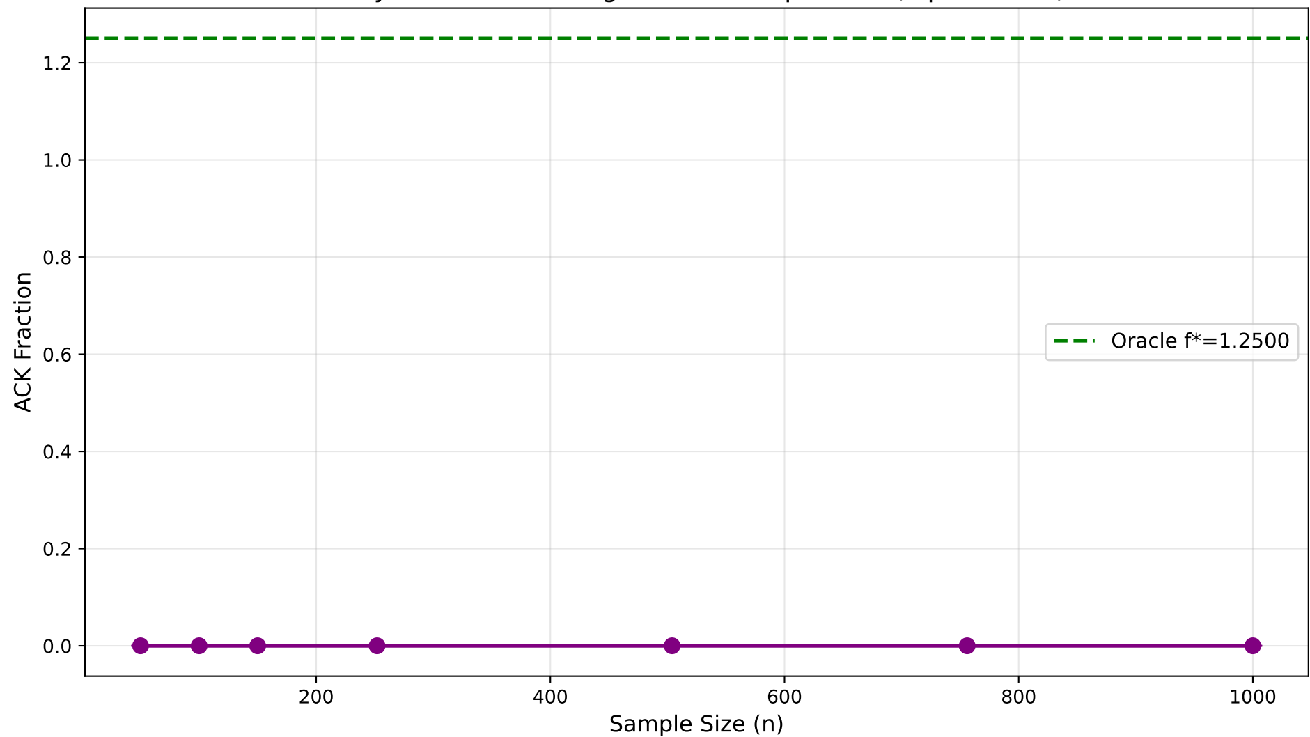
Kelly Fraction Convergence vs Sample Size ( \alpha=0.10 )
