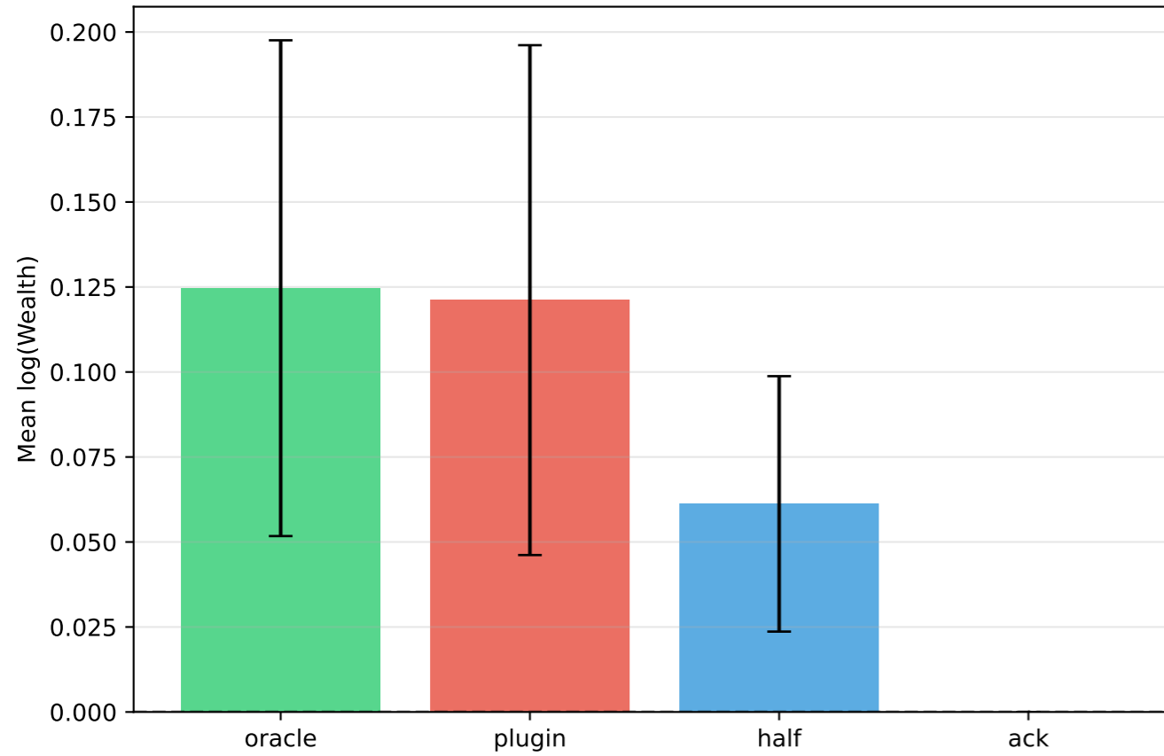
GARCH Returns
