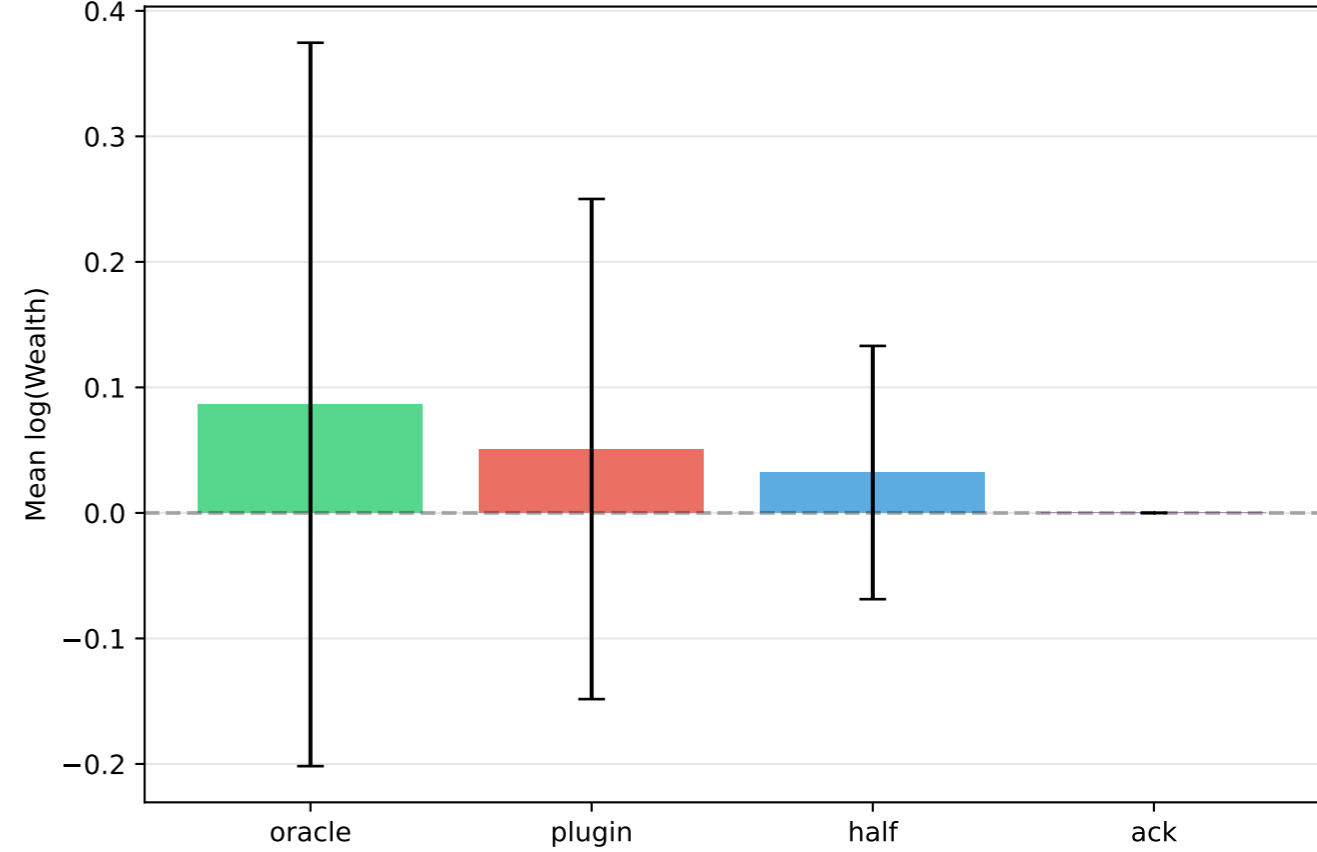
Jump-Diff Returns
