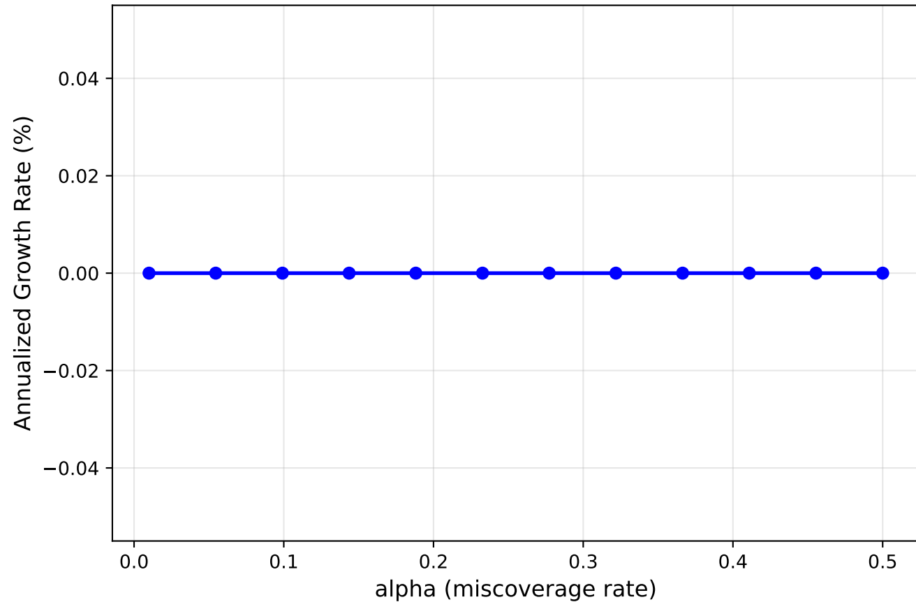
Growth Rate vs Confidence Level
