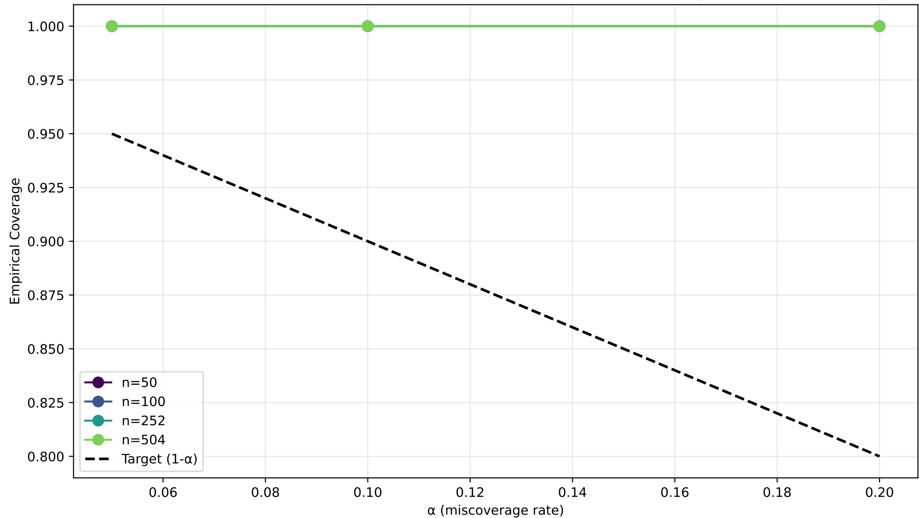
Theorem 2 Verification: Conformal Calibration Coverage
