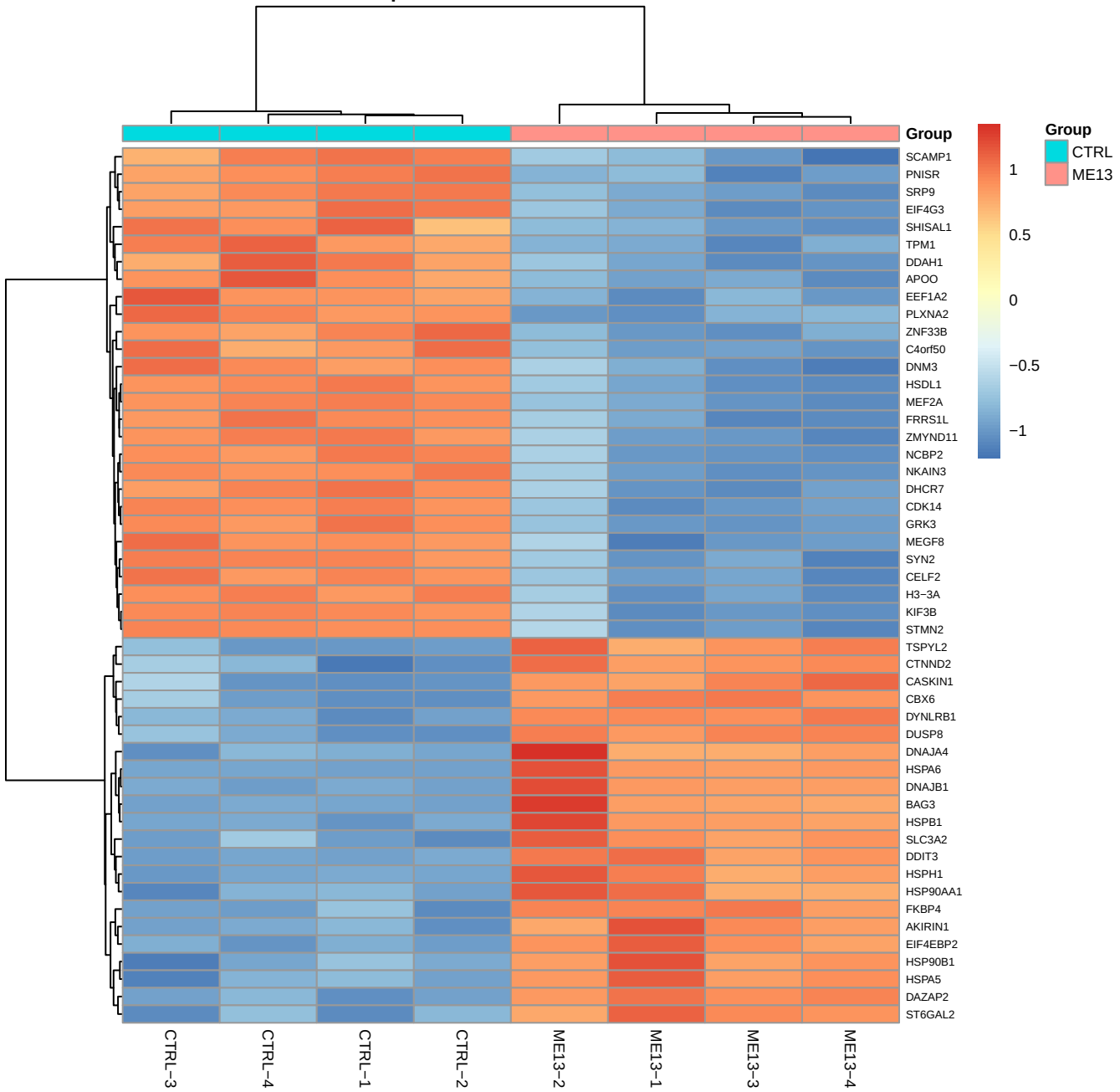
Top 50 DEGs: ME13_vs_CTRL
