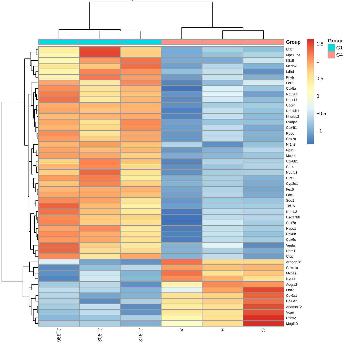
Top 50 DEGs: G1_vs_G4
