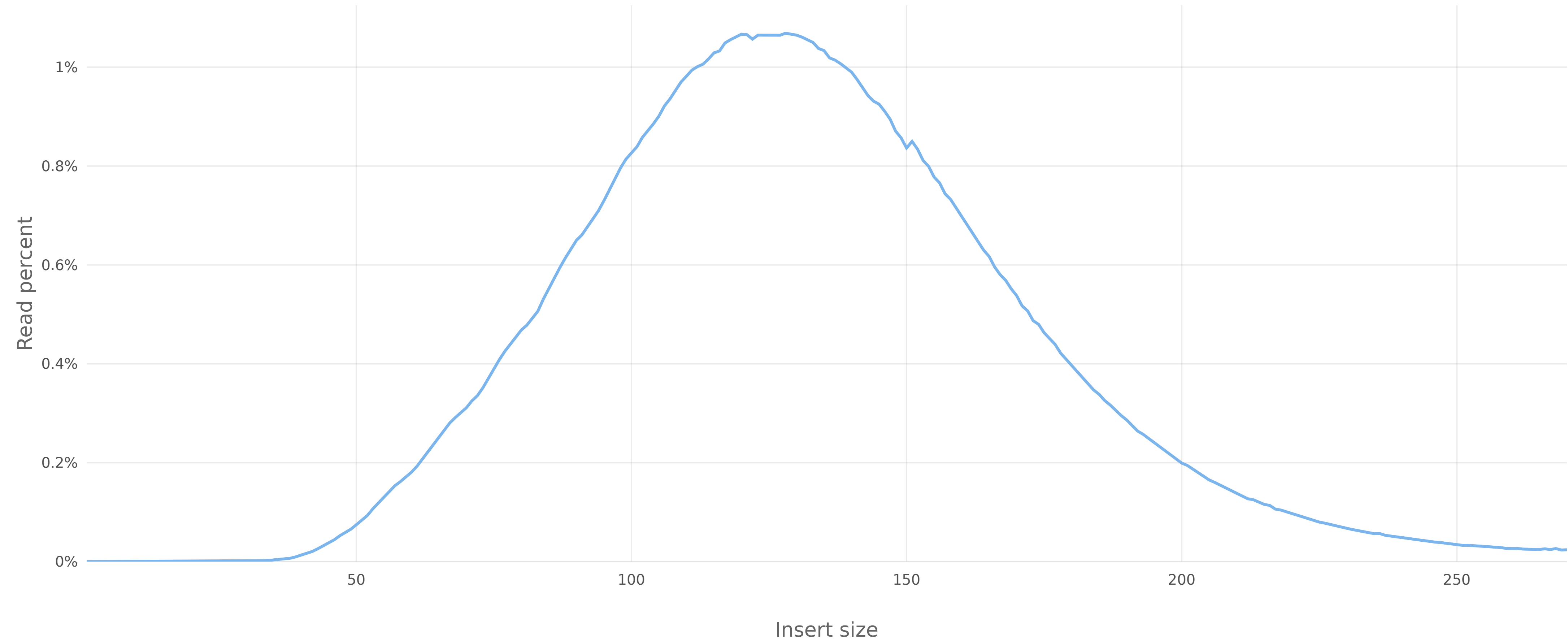
Fastp: Insert Size Distribution
