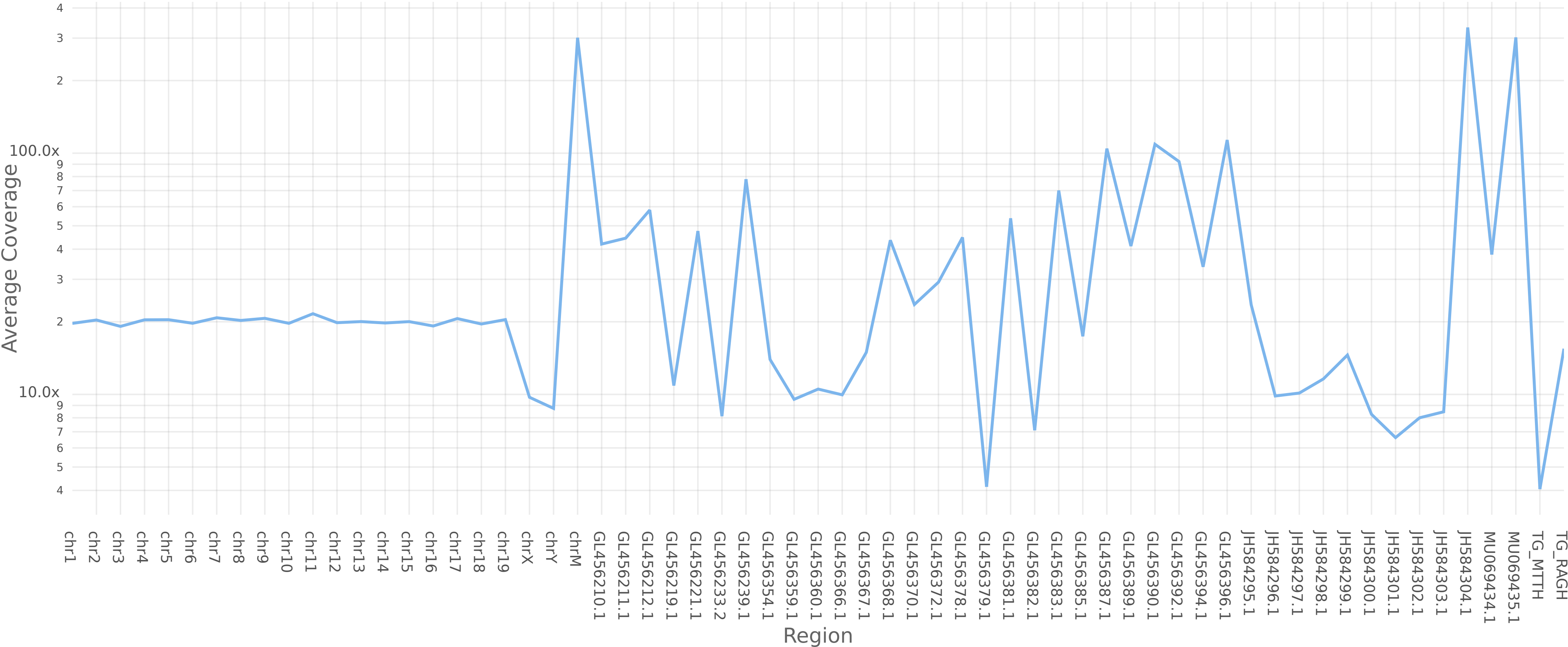
Mosdepth: Coverage per contig
