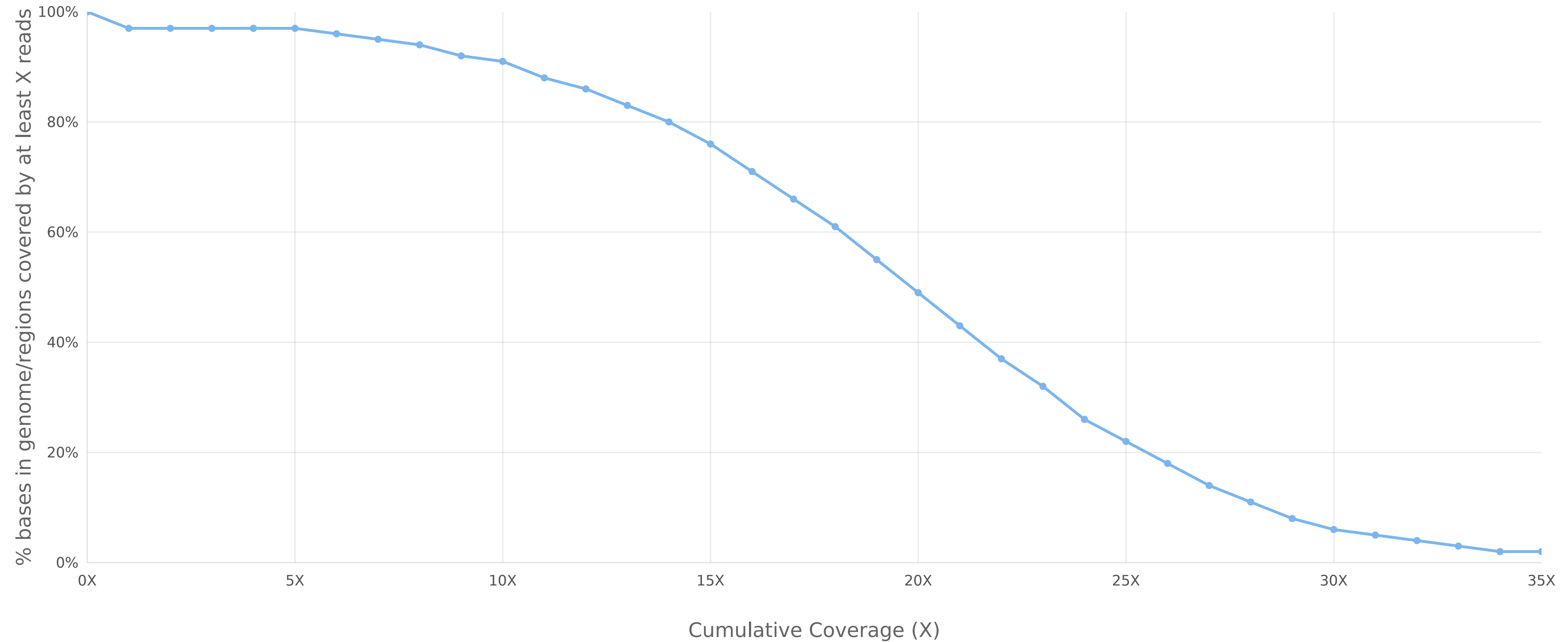
Mosdepth: Cumulative coverage distribution
