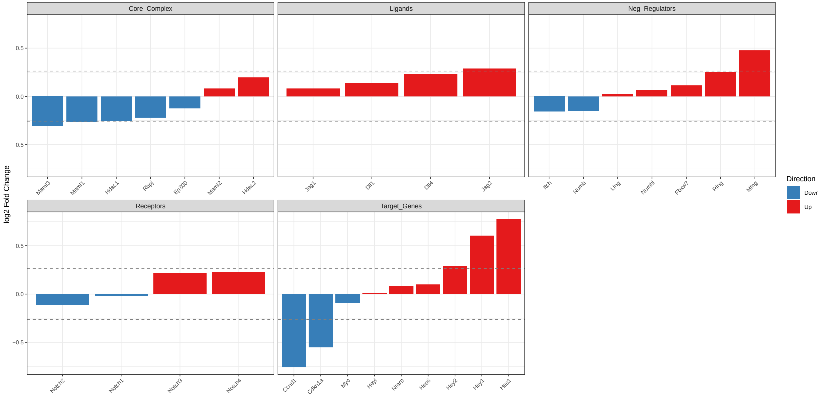
Notch Pathway Genes: G1_vs_G4
