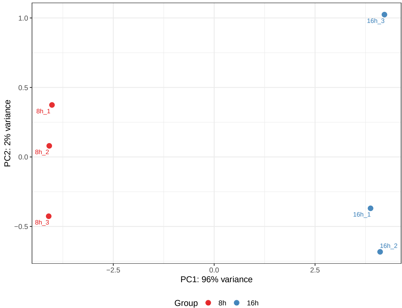
PCA – 8h vs 16h (current NovaSeq batch only, same-batch, reliable)
