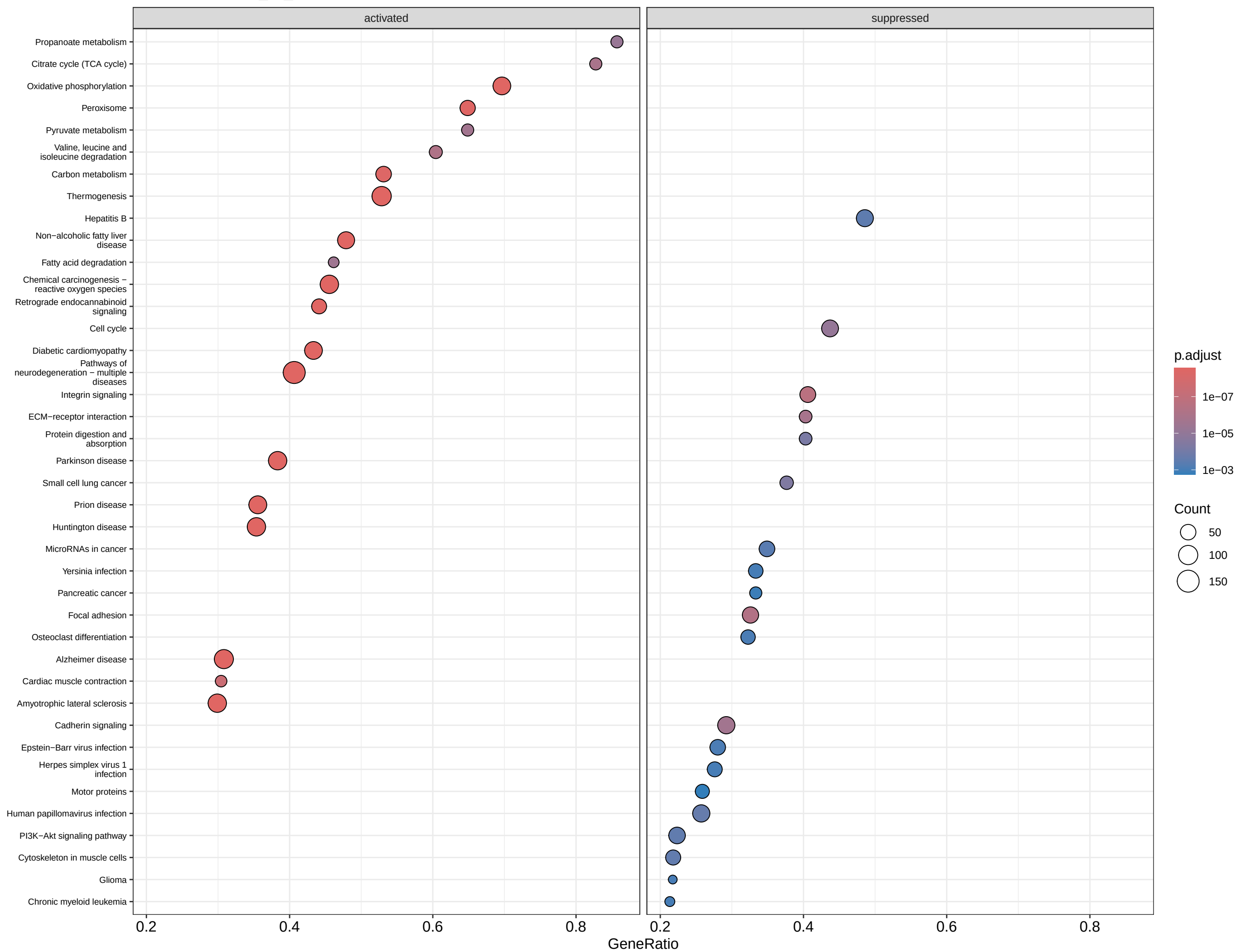
GSEA KEGG: G1_vs_G4
