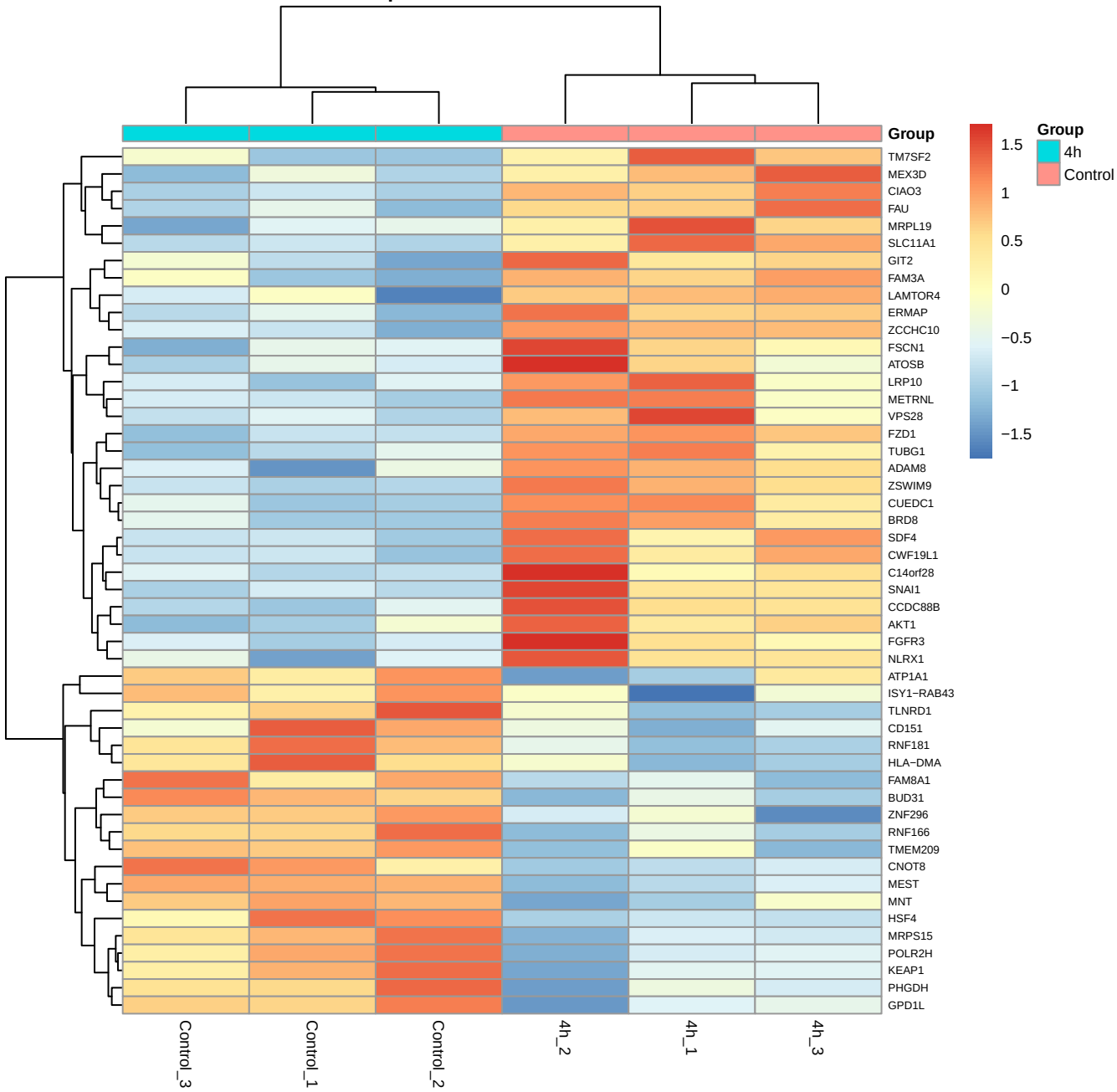
Top 50 DEGs: 4h_vs_Control
