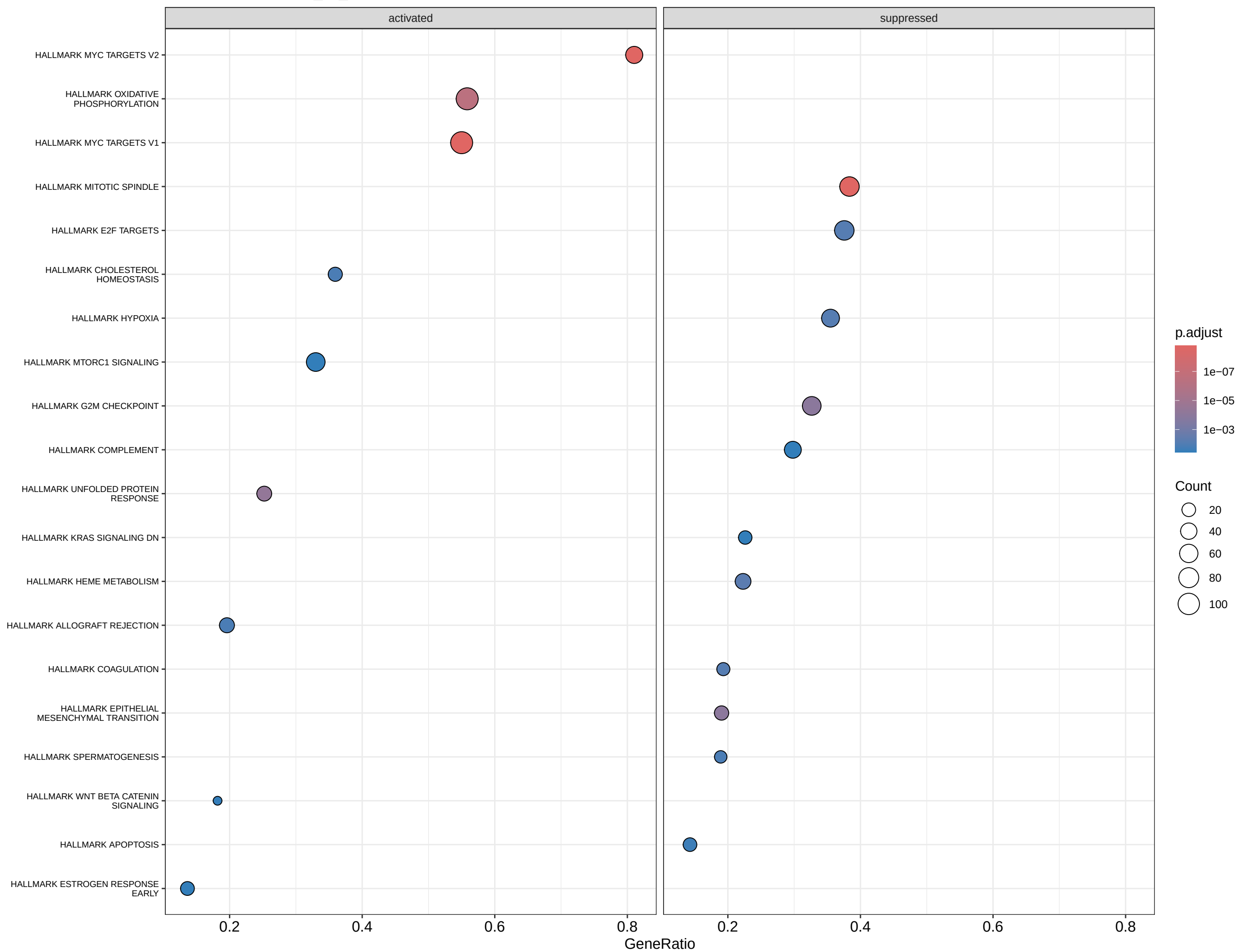
GSEA Hallmark: 16h_vs_8h
