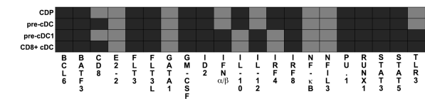
Fig. 3. Attractors of the Boolean model. Wild-type model attractors. Active nodes are marked in black, and inactive nodes in gray. The corresponding cell types are indicated in the leftmost column.
