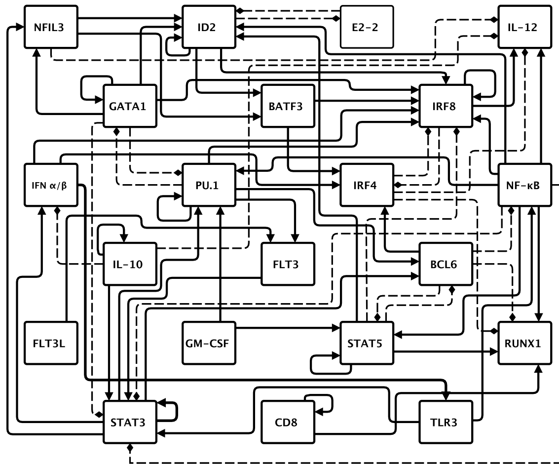
Fig. 2. The regulatory network controlling the differentiation of splenic CD8+ cDCs in mice. Nodes (black squares) represent molecules. Sharp continuous arrows represent activations, while blunt discontinuous arrows represent inhibitions.
