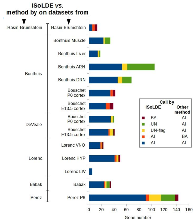
Fig. 2. Comparison of ISoLDE to other published methods on a series of experimental datasets. The indicated datasets were analyzed in parallel by ISoLDE and by one of the indicated published methods. For each method comparison, the genes called parentally biased ('AI') by either method were classified according to the calls of the two methods. 'AI', allelic imbalance. 'BA', bi-allelically expressed. 'UN', undetermined. 'UN-flag', undetermined and flagged by ISoLDE. The AI-AI pair in legend denotes genes called parentally biased by both ISoLDE and the compared method. The AI-BA and BA-AI pairs in legend denote genes called parentally biased by one method and bi-allelically
