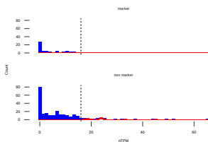
MUSK7, Cell type class of TF marker : Lung
