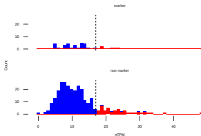
NUX3-1, Cell type class of TF marker : Prostate
