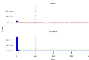
KLF2, Cell type class of TF marker : Liver
