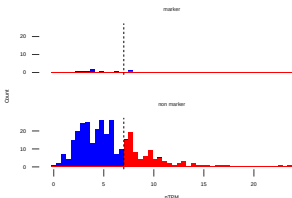
KLF7, Cell type class of TF marker : Lung
