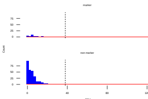
SOX1, Cell type class of TF marker : Breast
