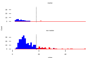
ELF1, Cell type class of TF marker : Breast
