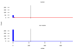
XBCCL, Cell type class of TF marker : Liver
