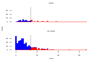
SATB1, Cell type class of TF marker : Lung
