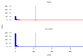
DCMES, Cell type class of TF marker : Liver
