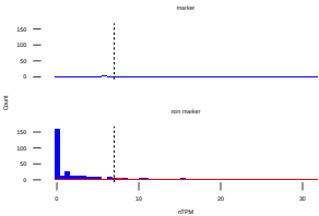
RP4, Cell type class of TF marker : Blood
