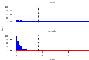
BRCA2, Cell type class of TF marker : Prostate
