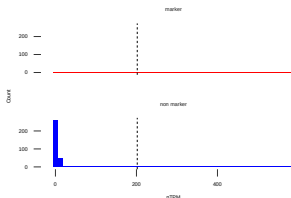
RNDML, Cell type class of TF marker : Lung
