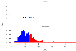
ULK3, Cell type class of TF marker : Breast
