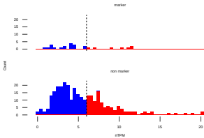
MESP1, Cell type class of TF marker : Lung
