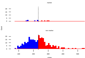
ATM, Cell type class of TF marker : Breast
