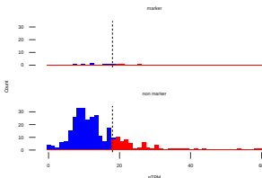
TEADOL, Cell type class of TF marker : Uterus
