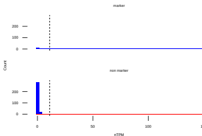
RSEBL, Cell type class of TF marker : Liver
