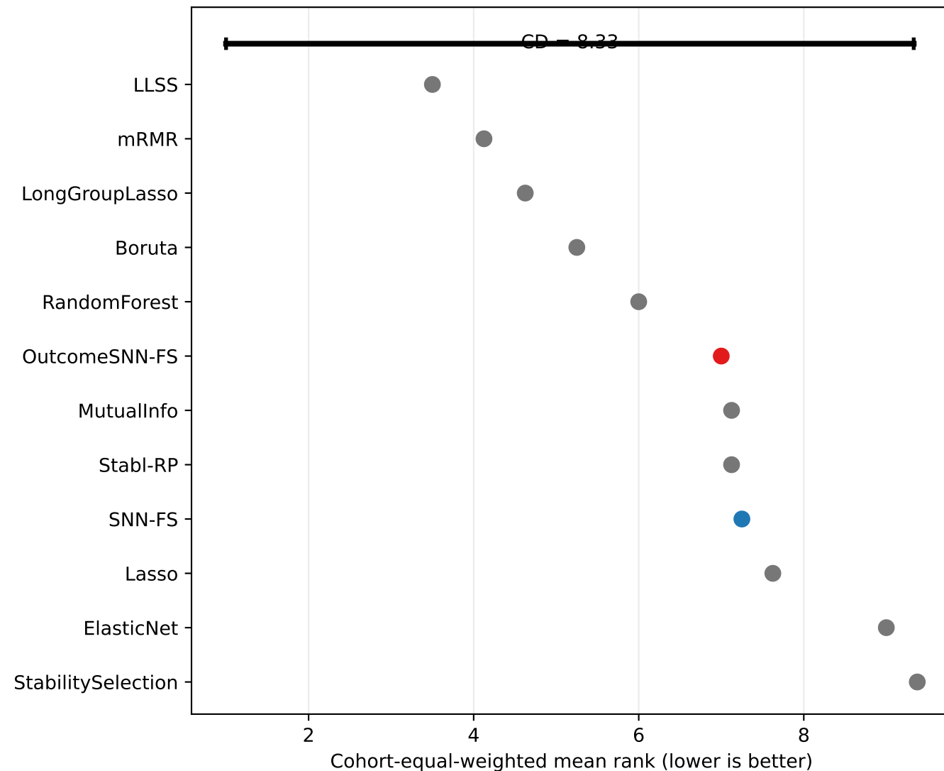
Classification: 4 source cohorts
