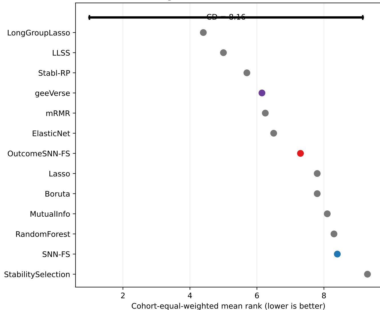
Regression: 5 source cohorts
