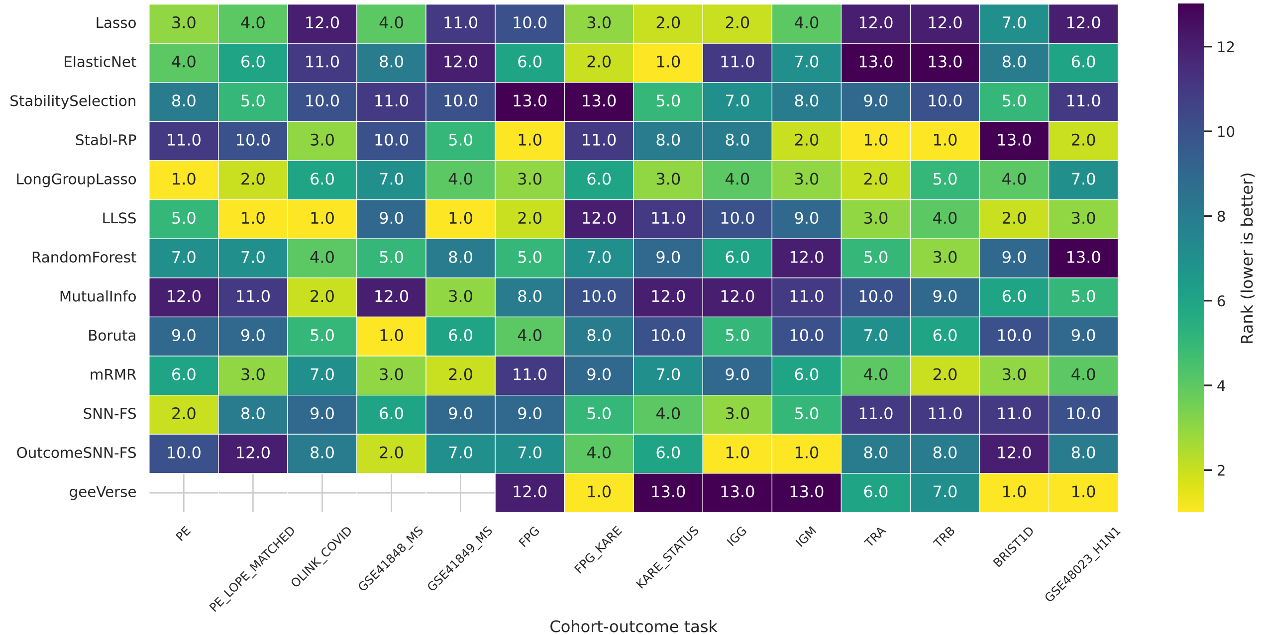
Method ranks vary across longitudinal biomedical tasks
