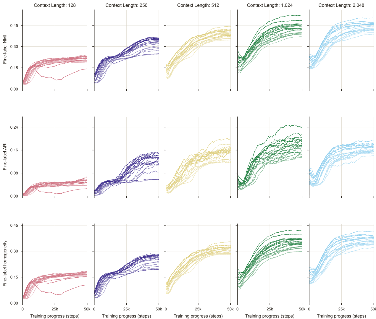
Binned Gene Expression: downstream metric trajectories
