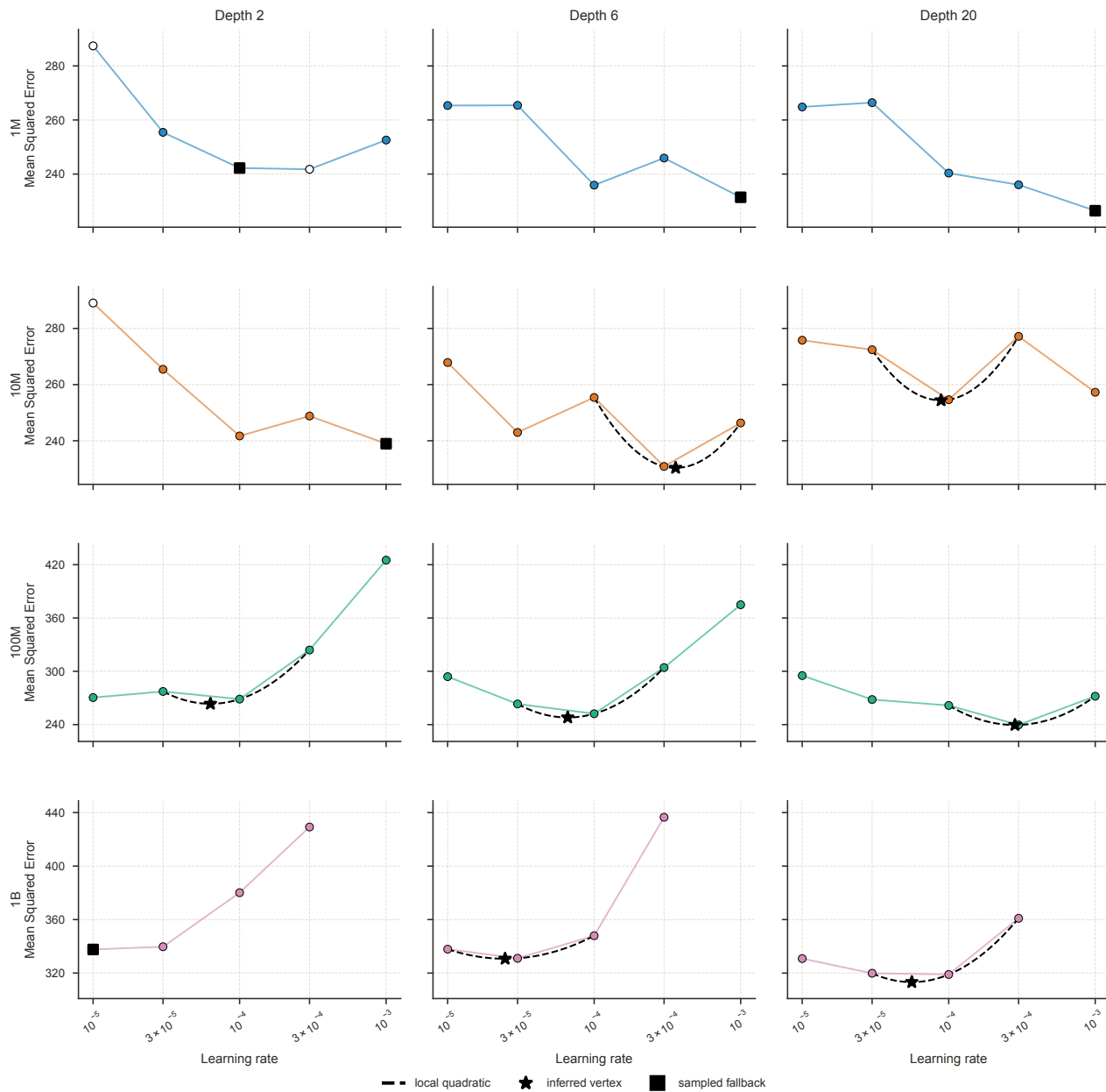
Binned Gene Expression: learning-rate sweeps at 1.05e+17 FLOPs
