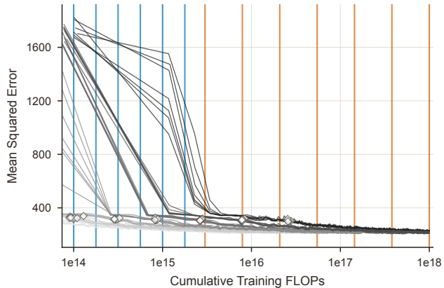
Binned Gene Expression
