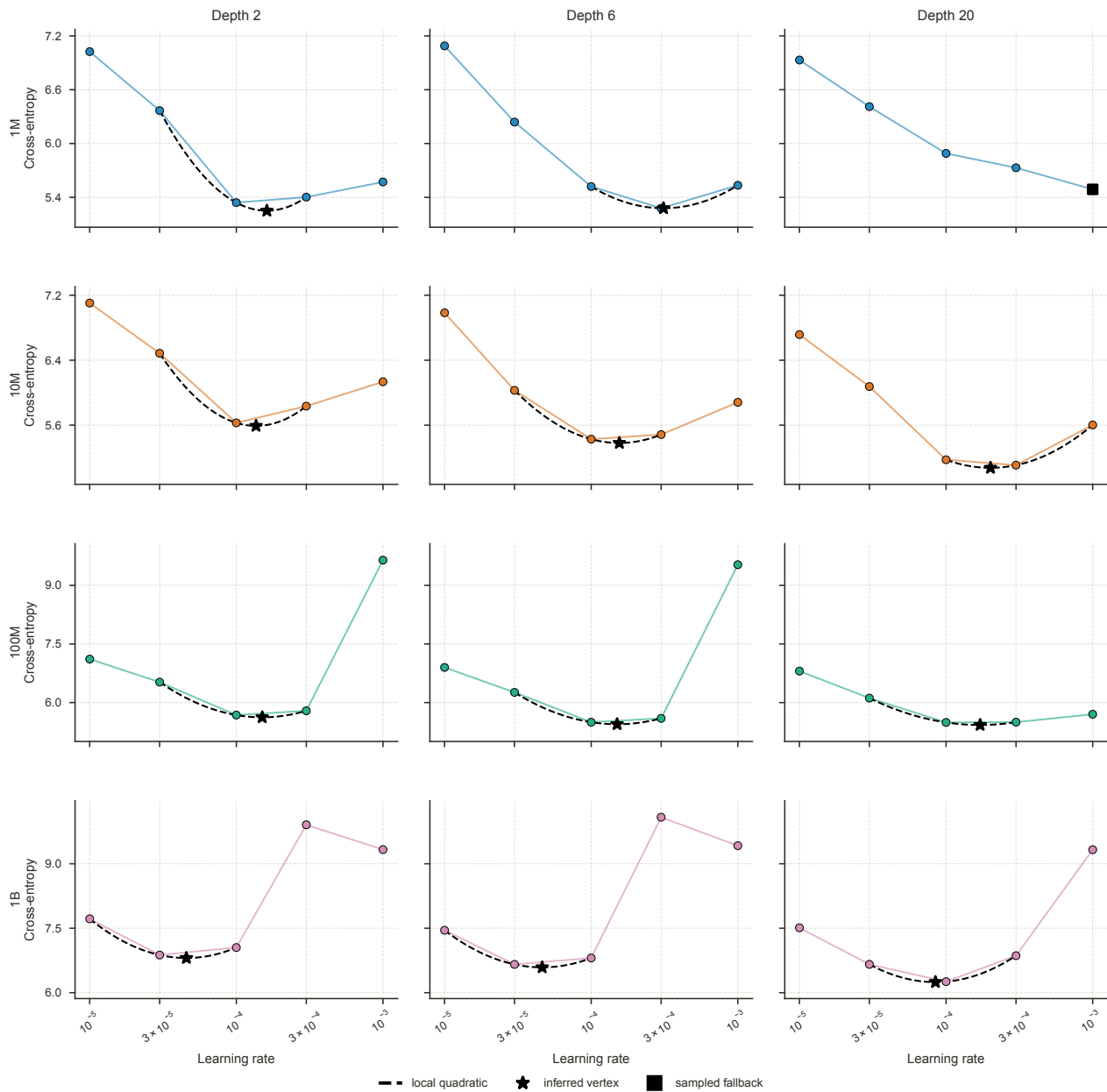
Ranked Gene Identity: learning-rate sweeps at 5.25e+17 FLOPs
