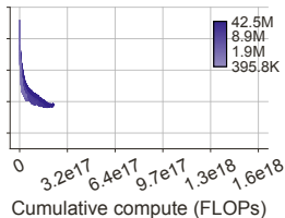
Context Length: 1024
