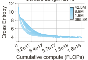
Context Length: 2048
