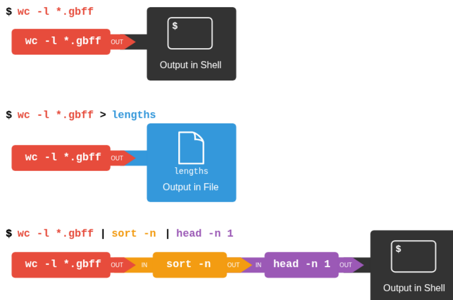
Figure 6.1: redirects_and_pipes
