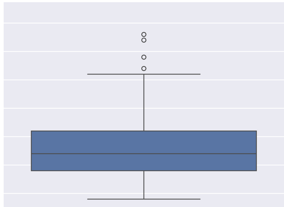
benchmarking
