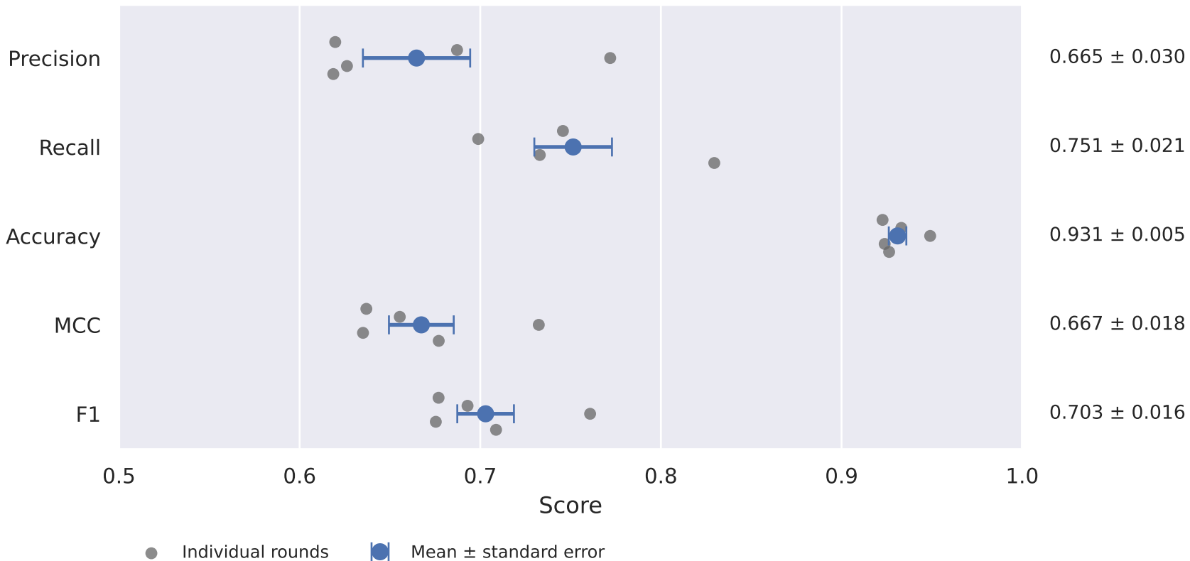
Von Heijne — performance on the five test folds
