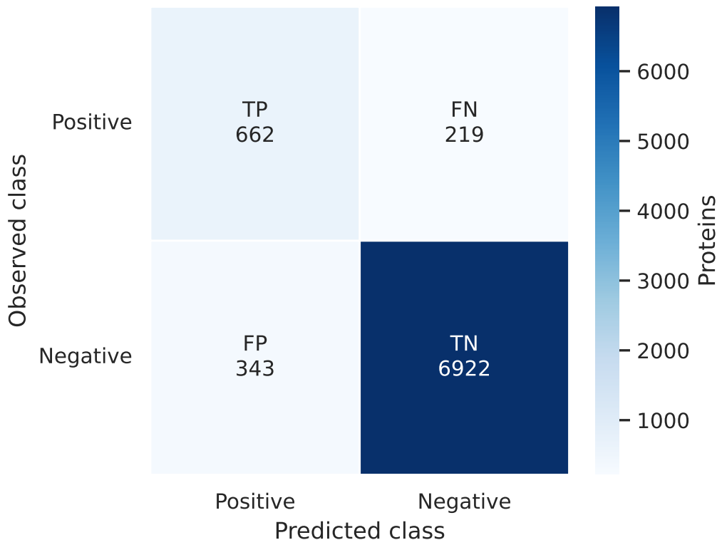
Pooled test-fold confusion matrix (5 rounds)
