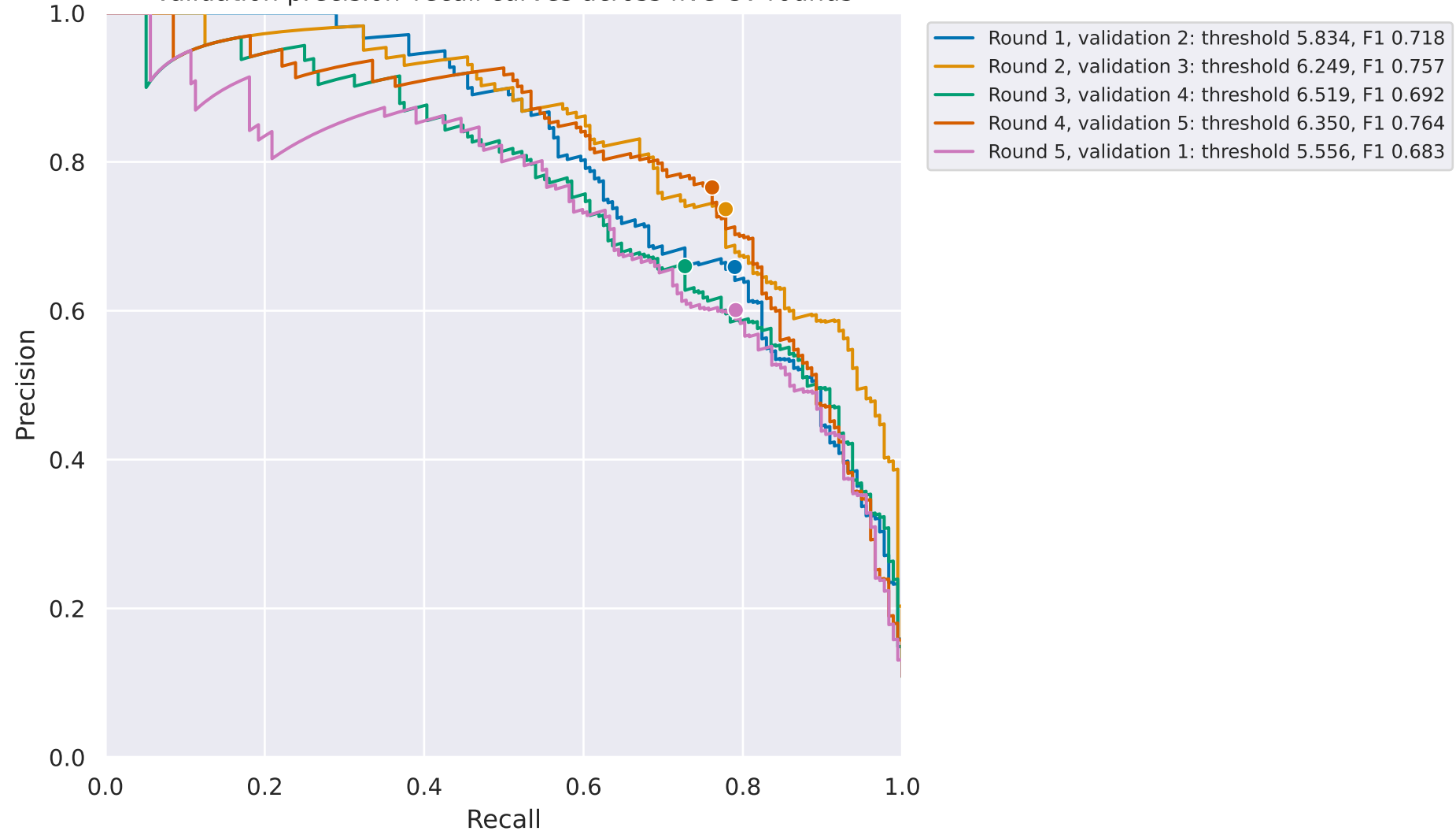
Validation precision-recall curves across five CV rounds
