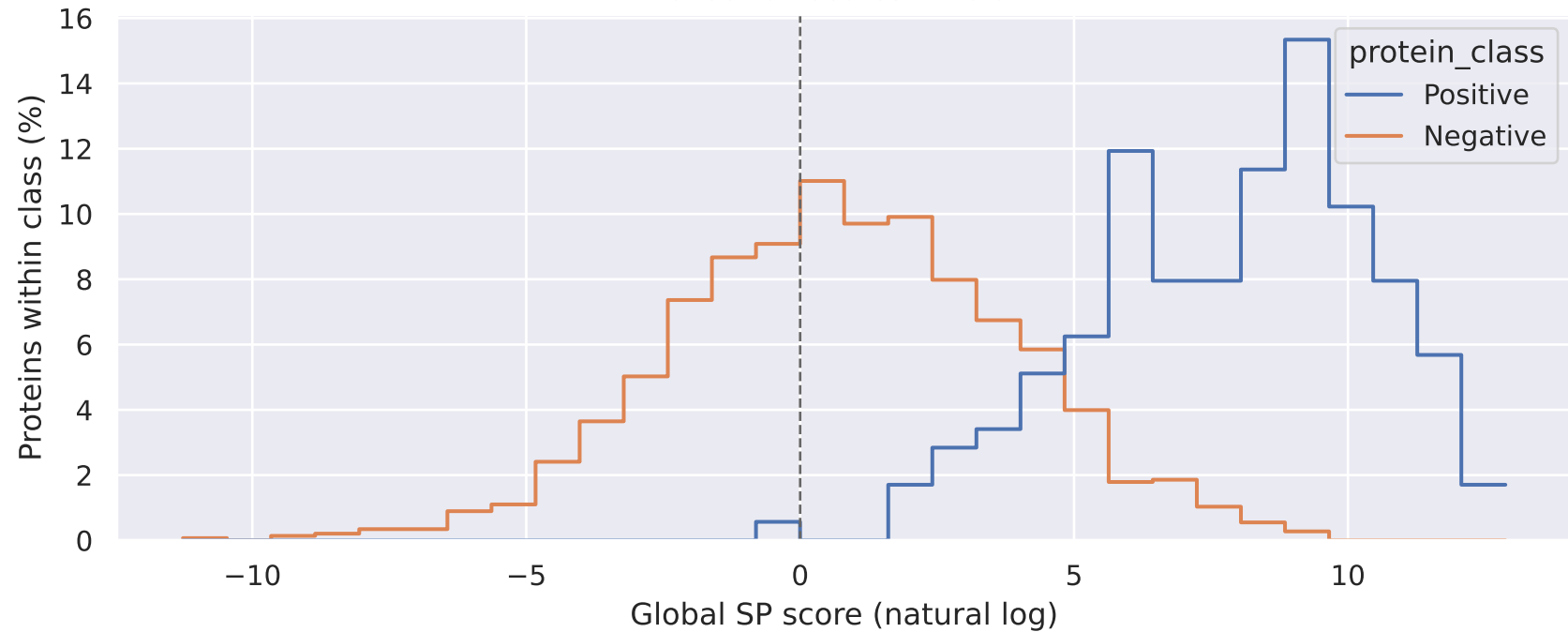
Validation scores — fold 2
