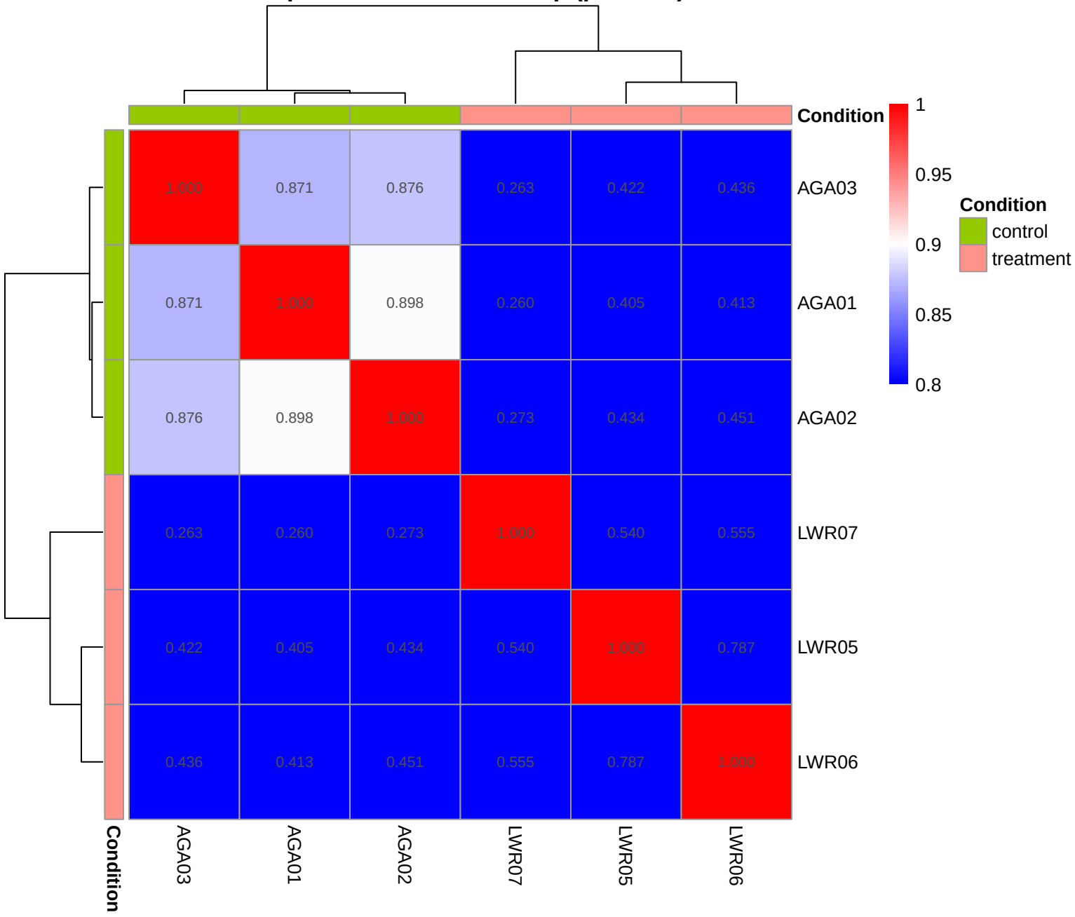
Sample Correlation Heatmap (pearson)
