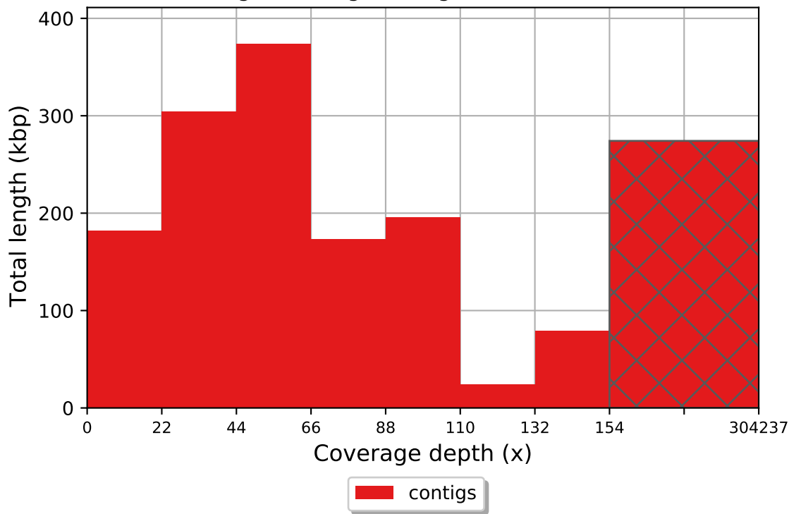
contigs coverage histogram (bin size: 22x)
