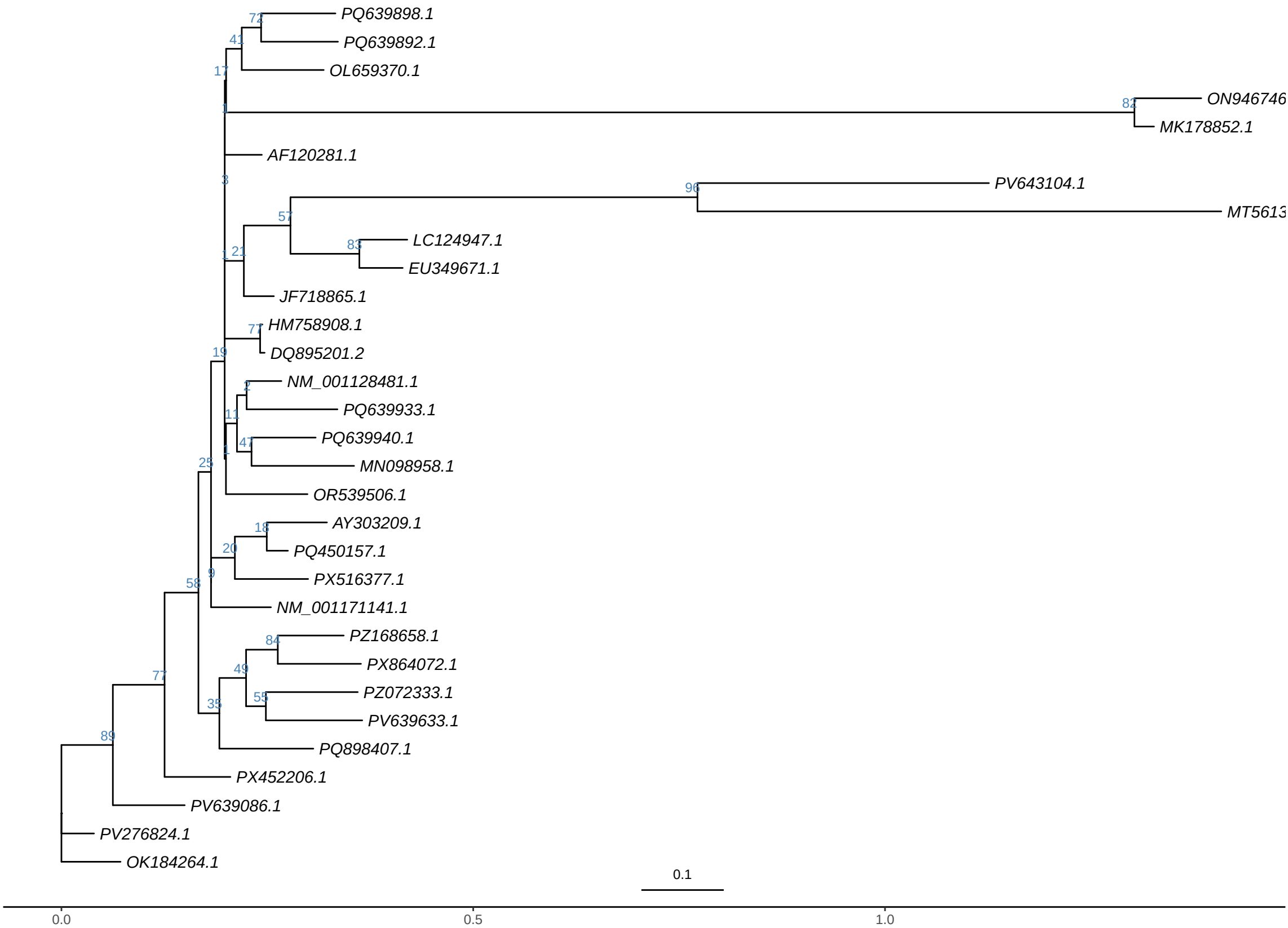
Supermatrix Species Tree (IQ-TREE)
